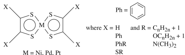
FIGURE 1 The molecular structure of transition metal dithiolenes. The physical properties of the complex are determined by the nature of the terminal functional groups, designated as X.
