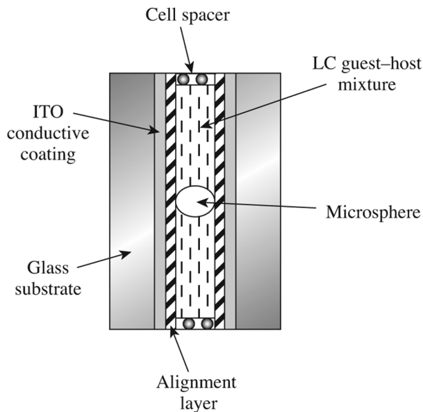
FIGURE 8 A schematic representation of the liquid crystal point diffraction interferometer (LCPDI) device.
