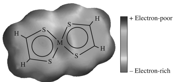
FIGURE 2 Ground-state charge distribution map of the nickel dithiolene core. The sulfur and nickel atoms are the most electron-rich areas in the molecule.
