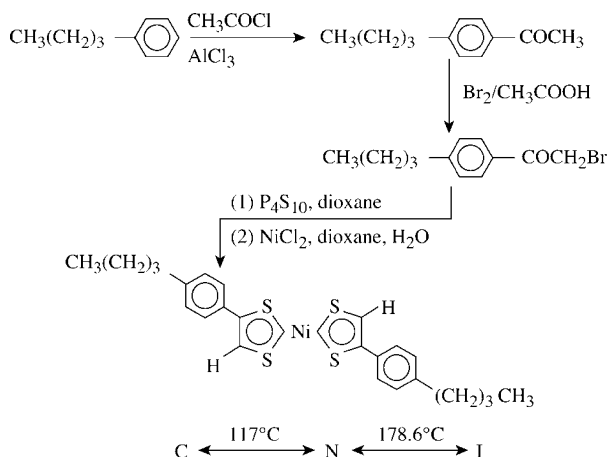
FIGURE 4 The synthesis method for rod-like nickel dithiolene compounds possessing a liquid crystal phase.
