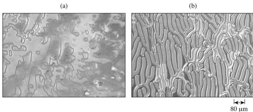
FIGURE 7 Chirality transfer to an LC host by host by doping with a chiral nickel dithiolene complex. (a) Pure Merck E7 and (b) Merck E7 containing 0.5% of the S-(+)-2 methylbutyritioether-substituted nickel dithiolene.
