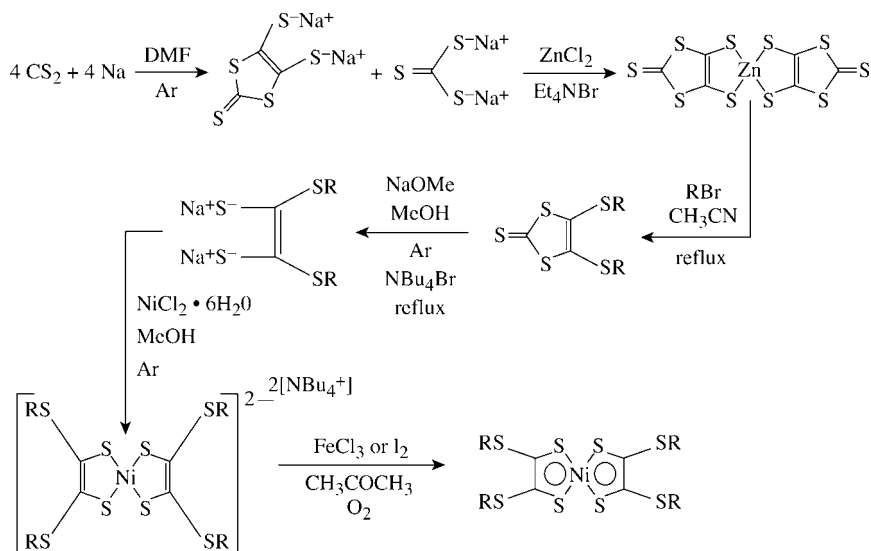
FIGURE 5 Modified synthesis scheme for preparation of tetrakis(alkylthio) bis(ethylene-1,2-dithiolene) nickel (0) complexes. Modifications to the established literature procedures resulted in substantially improved yields of product.
