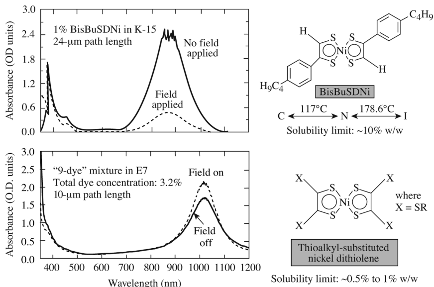
FIGURE 3 Change in absorbance with applied voltage at 860 nm for a 1% concentration of “BisBuSDNi” in a 24-μm-thick, antiparallel rubbed cell. An OD of 3.5 is achievable at higher dye concentrations (top). Field-induced dichroic behavior of a mixture of nine thioalkyl-substituted nickel dithiolene dyes in Merck E7. Increasing the number of terminal substituents from two to four and altering their structure changes the sign of the dichroism from positive to negative (bottom).
