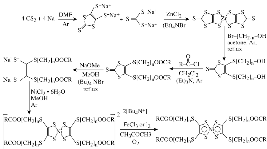
FIGURE 6 Synthesis scheme for chiral transition metal dithiolenes incorporating a flexible spacer between the terminal groups and the dithiolene core.
