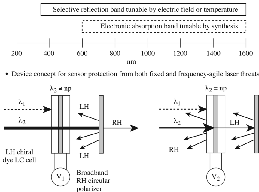
FIGURE 9 Device concept for sensor protection in the near IR based on chiral nickel dithiolene dyes. The device has two modes of tunability: one mode through the absorbance of the nickel dithiolene dye (tunable by synthesis) and a second tunable mode employing selective reflection wavelength shifting induced by electric field or temperature changes.
