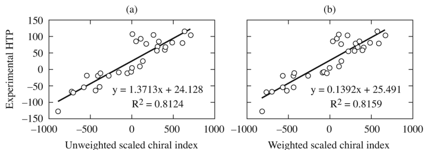
FIGURE 10 The weighted (a) and unweighted (b) scaled chiral indices of all 32 rigid molecules plotted against the experimental helical twisting power data. A linear regression is used to determine the strength of the correlation. The R^2 value of the weighted index (0.82) is slightly stronger than that of the unweighted index (0.81).
